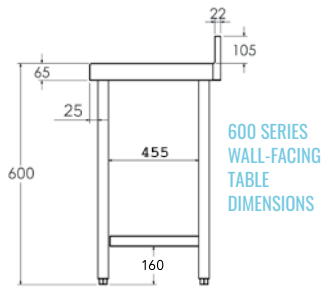
600 SERIES CENTER TABLE DIMENSIONS
