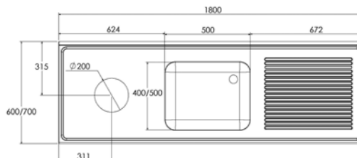
INDUSTRIAL SINK DIMENSIONS 1800 MM
