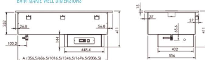
BAIN-MARIE WELL DIMENSIONS
