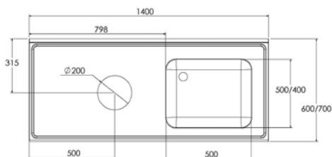
INDUSTRIAL SINK DIMENSIONS 1400 MM
