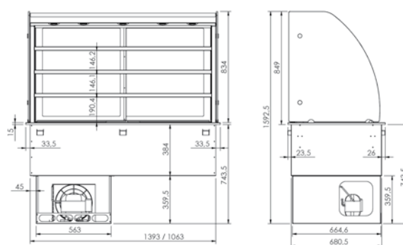
GLASS DISPLAY CASE DIMENSIONS
