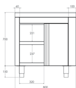
NEUTRAL SELF-SERVICE WITH SWINGING DOORS DIMENSIONS
