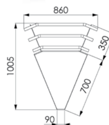
MODEL S1000412 DIMENSIONS
