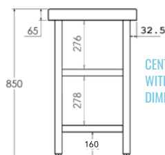
CENTER TABLE WITH SHELF DIMENSIONS
