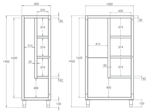
FREESTANDING CABINET DIMENSIONS
