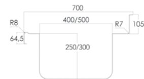
BASIN DIMENSIONS
