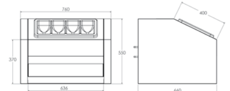
DISPENSER DIMENSIONS
