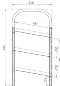
TROLLEY DIMENSIONS
