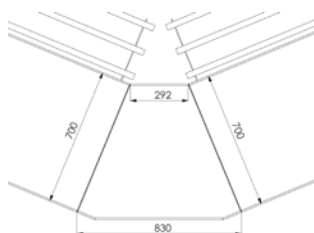
MODEL S1000411 DIMENSIONS
