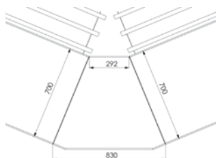
MODEL S1000411 DIMENSIONS
