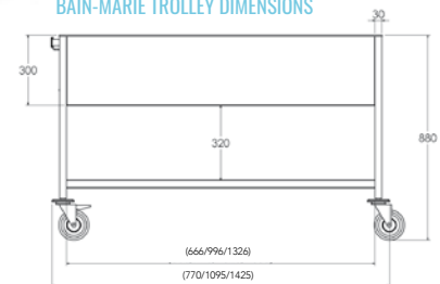
BAIN-MARIE TROLLEY DIMENSIONS
