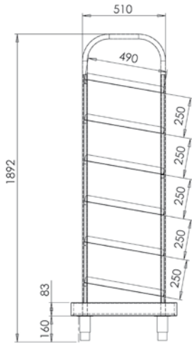
TROLLEY DIMENSIONS
