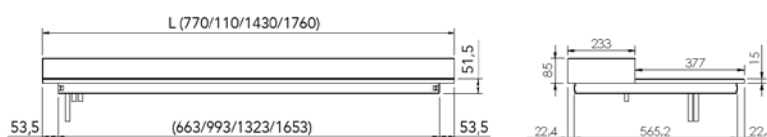
TWO-LEVEL COLD PLATE DIMENSIONS
