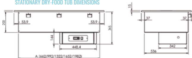
STATIONARY DRY-FOOD TUB DIMENSIONS
