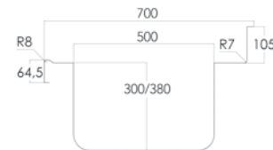
BASIN DIMENSIONS
