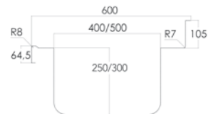
BASIN DIMENSIONS
