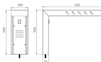
STRIP WARMER DIMENSIONS
