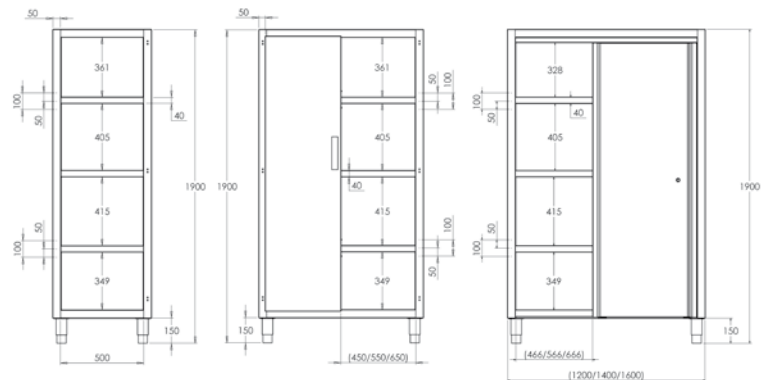
FREESTANDING CABINET DIMENSIONS
