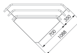
MODEL S1000402 DIMENSIONS
