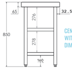
CENTER TABLE WITH SHELF DIMENSIONS
