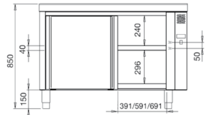
HOT FOOD TABLE DIMENSIONS
