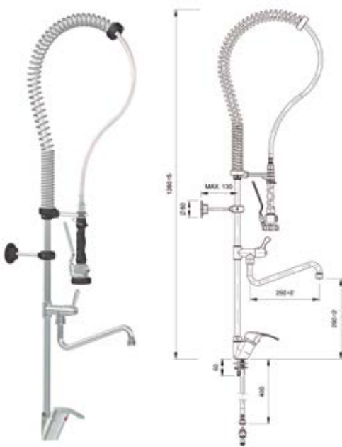
Model Code Single-handle Spraying tap with extra tap • R0020302
