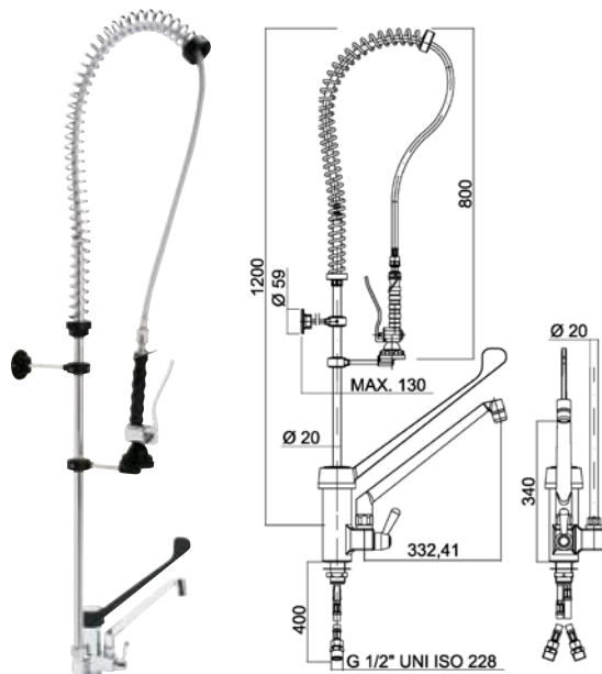
Model Code Spraying tap with hot/cold controls and extra tap • R0020301
