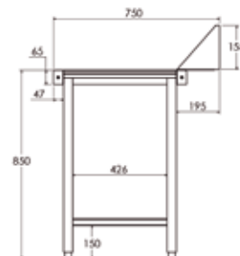
WALL-FACING TABLE DIMENSIONS
