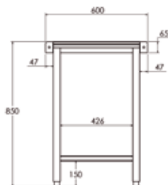
CENTER TABLE DIMENSIONS
