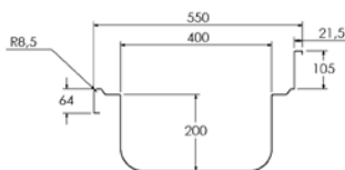
BASIN DIMENSIONS
