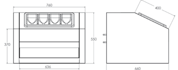
DISPENSER DIMENSIONS
