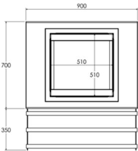
SELF-SERVICE NEUTRAL DISH RACK DISPENSER DIMENSIONS
