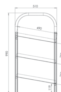
TROLLEY DIMENSIONS
