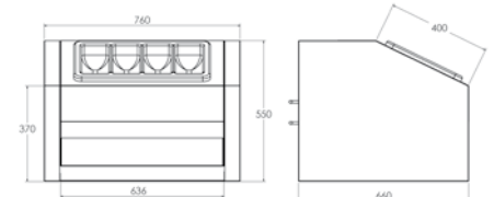
DISPENSER DIMENSIONS
