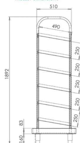
TROLLEY DIMENSIONS
