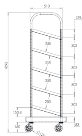
TROLLEY DIMENSIONS
