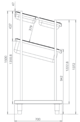
DISPENSER DIMENSIONS
