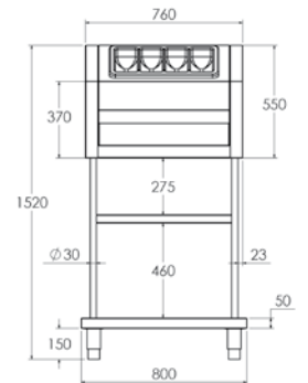
DISPENSER DIMENSIONS
