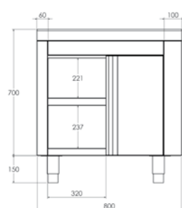
NEUTRAL SELF-SERVICE WITH SWINGING DOORS DIMENSIONS
