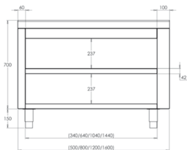
NEUTRAL SELF-SERVICE WITH SHELF DIMENSIONS
