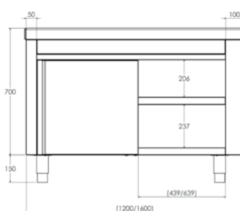
NEUTRAL SELF-SERVICE WITH SLIDING DOORS DIMENSIONS
