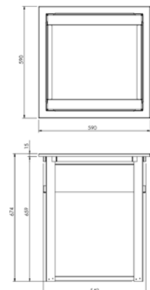
NEUTRAL DISH RACK DISPENSER DIMENSIONS
