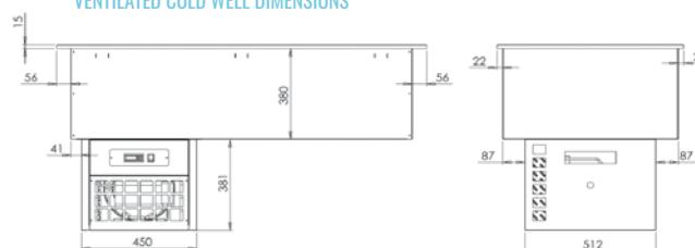
VENTILATED COLD WELL DIMENSIONS
