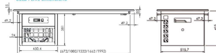
COLD PLATE DIMENSIONS
