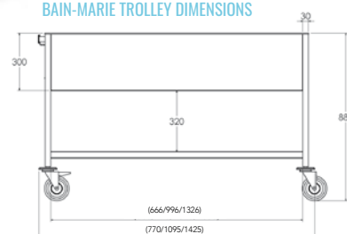
BAIN-MARIE TROLLEY DIMENSIONS
