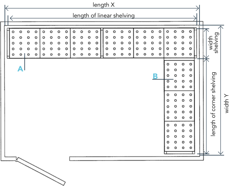
Linear shelving (A)
