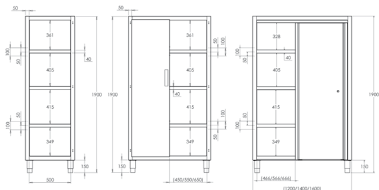
FREESTANDING CABINET DIMENSIONS
