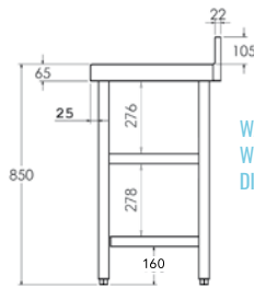
WALL-FACING TABLE WITH SHELF DIMENSIONS
