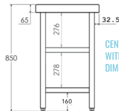
CENTER TABLE WITH SHELF DIMENSIONS
