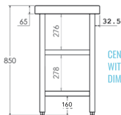
CENTER TABLE WITH SHELF DIMENSIONS
