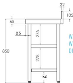
WALL-FACING TABLE WITH SHELF DIMENSIONS
