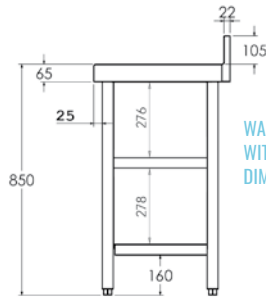
WALL-FACING TABLE WITH SHELF DIMENSIONS
